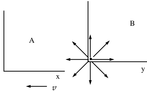
Figure 1.5: E(y) = Q/y^2 .
