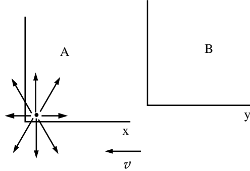
Figure 1.4: E(y) = Q/y^2 .
