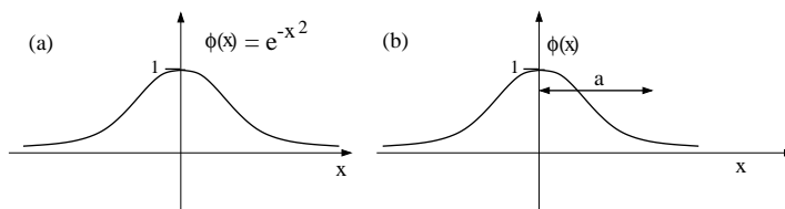
Figure 1.14: Illustration of smearing. operator valued distributions.
