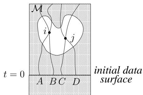
Figure 1.13: Resolution of Einstein's hole argument.
