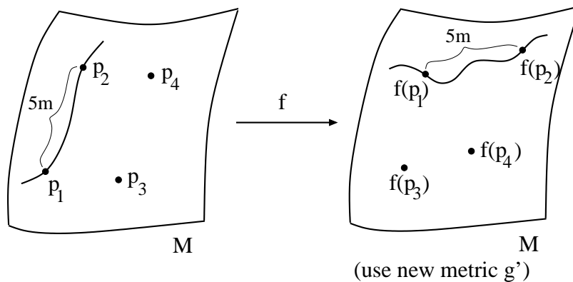
Figure 1.6: Passive spatial diffeomorphism f : M \rightarrow M refers to invariance under change of coordinates. The same object in a different coordinate system. Any theory of nature is invariant under passive diffeomorphisms.
