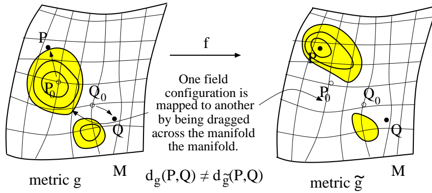
Figure 1.7: An active diffeomorphism f : M \rightarrow M drags fields on the manifold while remaining in the same coordinate system. f is viewed as a map that associates one point in the manifold to another one.
