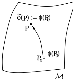
Figure 1.8: The value of \tilde{\phi}(P) at P is equated to the value of \phi(P_0) at P_0 , i.e. \tilde{\phi}(P) = \phi(P_0) . Under this transformation f we identify one point of the manifold P_0 to another point P f : P_0 \rightarrow P .
