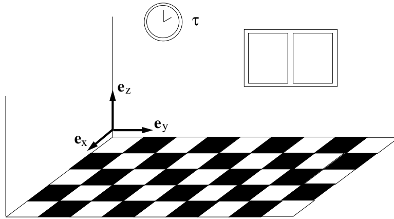
Figure 1.16: Laboratory walls exemplify Newton's absolute space and the clock absolute time. We can define positions relative to the wall.
