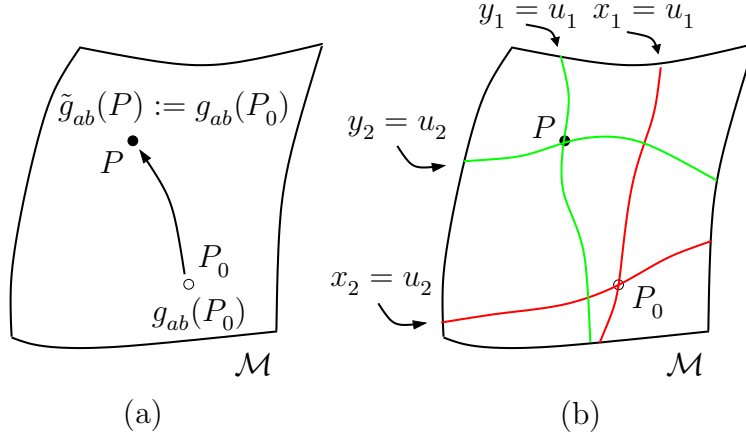
Figure 1.9: The value of the metric function \tilde{g}_{ab} at P is defined by the value of the metric function g_{ab} at P_0 , i.e. \tilde{g}_{ab}(P) = g_{ab}(P_0) . We go to a new coordinate system which assigns P the same coordinate values that P_0 has in the x -coordinates, so that \tilde{g}_{ab}(y_1 = u_1, y_2 = u_2) = g_{ab}(x_1 = u_1, x_2 = u_2) , compare to (1.31).
