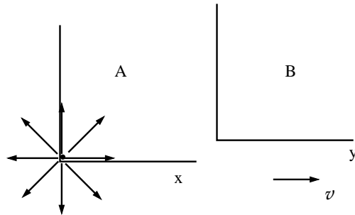
Figure 1.3: E(x) = Q/x^2 .
