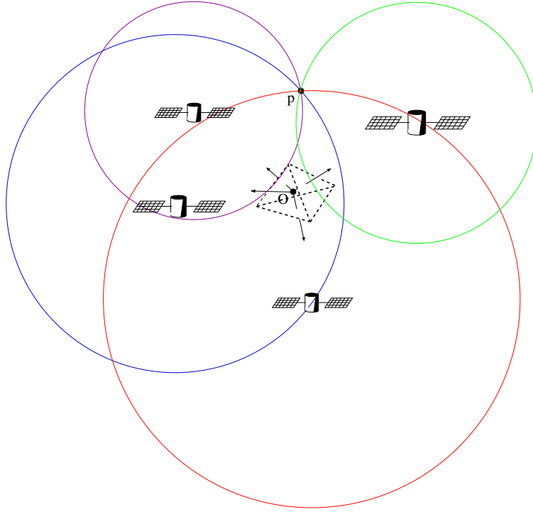
Figure 1.18: GPS3D A spacetime point in Minkowski spacetime can be expressed as a relation amongst 4? measurable variables. This definition of spacetime location retains meaning in the jump to GR.
