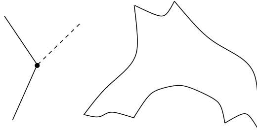
Figure 1.15: Regime where gravity is very strong so that the non-perturbative and background independence of GR must be taken into account. That spacetime points have no independent physical reality casts doubt on the hand-wavey argument I gave above.
