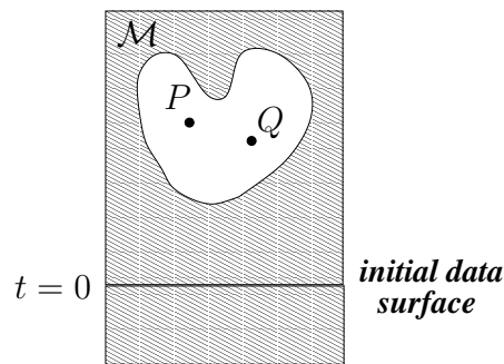
Figure 1.12: Einstein's hole argument.
