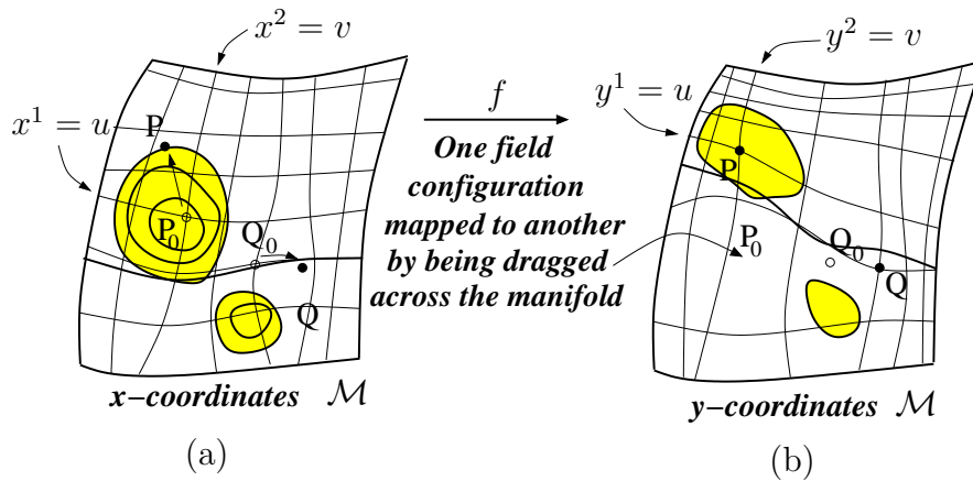
Figure 1.11: (a) An active diffeomorphism in which we actively drag the tensor function over the, in doing so identify one point of the manifold to another. (b) We then go to a coordinate system which assigns the newly identified points their original coordinate values. That is to say - we carry the tensor function over the manifold, keeping the coordinate lines ‘attached’.
